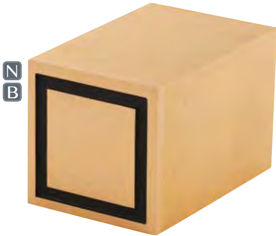
71010452 CUBE 5.5" H x 5.5" W x 8" D CAST FACE Volume: 218ci Access: Back
